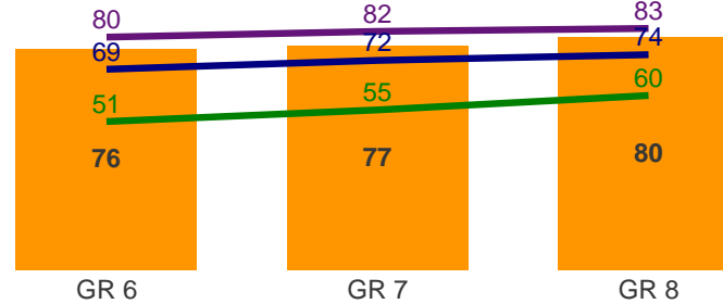
6-8 Reading Proficiency
