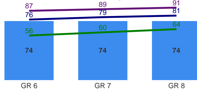
6-8 Math Proficiency
